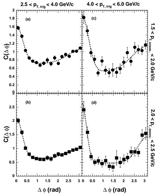
Fig. 1. d+Au correlation functions C(\Delta\phi) for several p_T selections as indicated. The centrality selection is 0-80%. The dashed line represents a double gaussian fit to the data.
